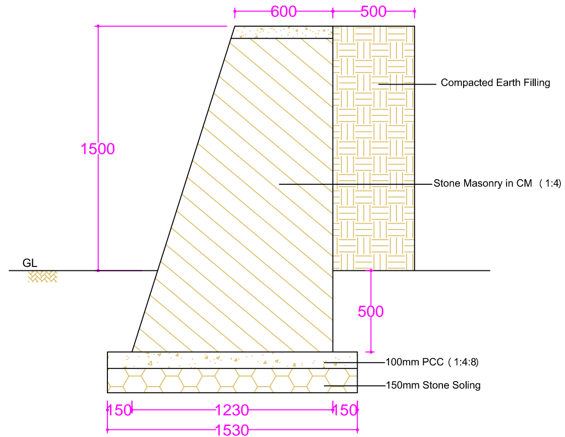
CROSS SECTION OF RETAINING WALL 1.50 M HEIGHT ( LENGTH - 27.70 M)
